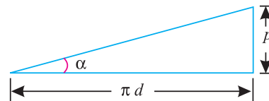
Fig. 9.21. Helix angle
