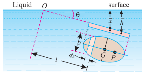
Fig. 35.12. Centre of pressure on an inclined immersed surface.
