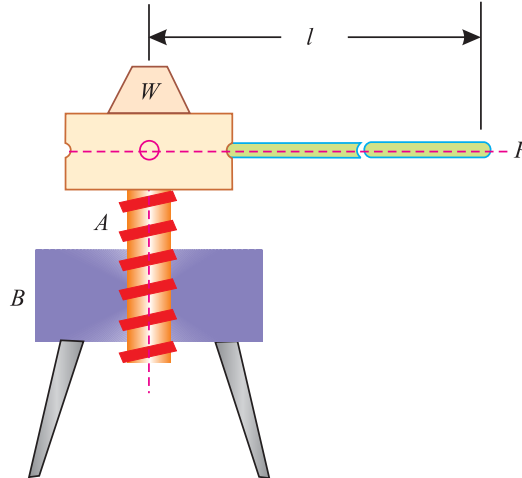
Fig. 9.20. Screw jack
