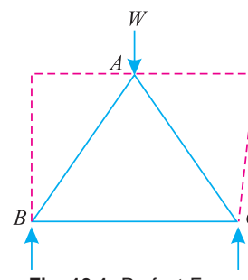
Fig. 13.1. Perfect Frame.
