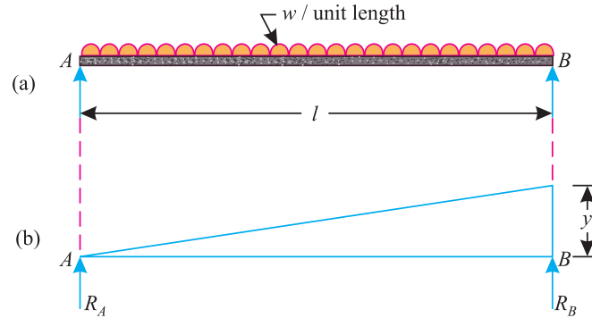
Fig. 16.8. Beam carrying uniformly distributed load.
