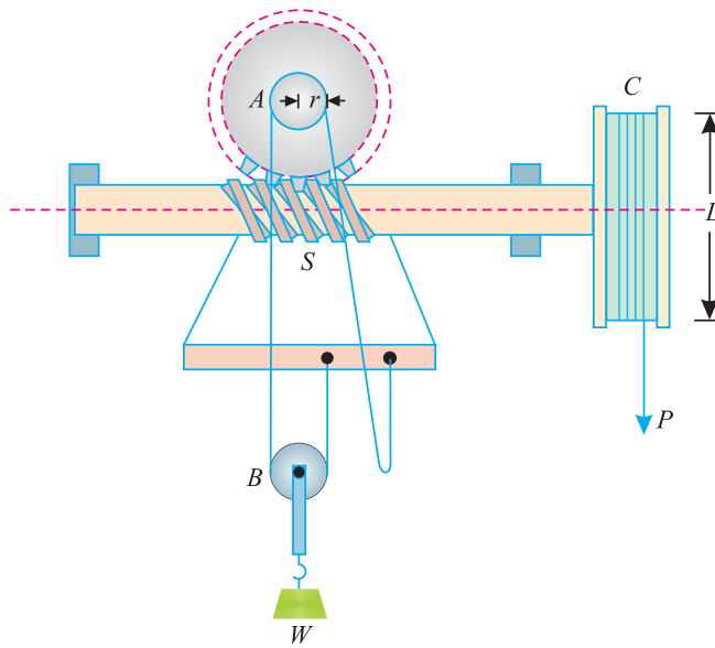
Fig. 11.6. Worm geared pulley block.
